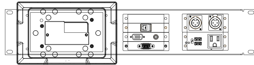
Crestron TSW-UMB-60 Touch Panel Back Box
