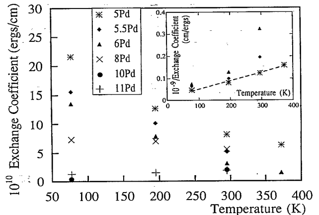
FIG. 4. FMR results of the exchange-coupling coefficient A^{AB} vs temperature in 5Fe/ x Pd/10Fe trilayers ( x=5,5.5, 6,8,10,11 ). FMR and BLS measurements probe an area 13 mm and 20 \mu\text{m} in diameter, respectively. BLS measurements at 295 K resulted in the same A^{AB} for the samples having 5, 6, 8, 10, and 11 Pd thick interlayers and gave a somewhat lower value (13%) for the sample having a 5.5 Pd interlayer. This agreement shows that the MBE-grown samples exhibit a uniform magnetic behavior.
