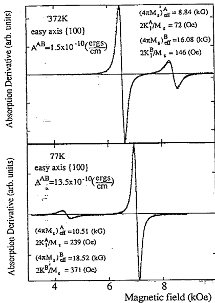
FIG. 3. The field derivative of FMR absorption at 36 GHz in the 5Fe/6Pd/10Fe trilayer (+) at 372 and 77 K. The solid line was calculated using the theory of exchange-coupled Fe layers (Ref. 10) with magnetic parameters (shown in figure) obtained from a \chi^2 fit. The magnetic parameters of individual 5Fe/8Pd and 8Pd/10Fe bilayers are (4\pi M_S)_{\text{eff}}^A = 9.05 and 10.71 kG, (4\pi M_S)_{\text{eff}}^B = 16.14 and 18.56 kG, 2K_1^A/M_S = 50 and 241 Oe, and 2K_1^B/M_S = 132 and 308 Oe at 372 and 77 K, respectively. A denotes the 5-ML Fe layer and B denotes the 10-ML Fe layer.
