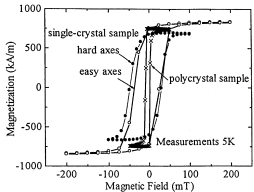
Fig. 2. Hysteresis curves for Fe/ \text{KMnF}_3 at 5 K. The samples were cooled in a field of 500 mT. The coercivity is substantially larger for the single-crystal sample.
