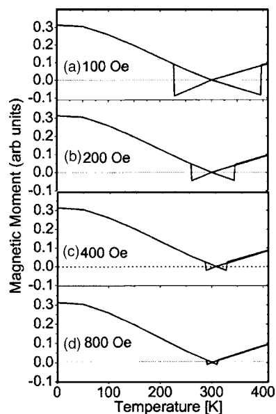
FIG. 2. Theoretical calculations for magnetization as a function of temperature for 2-nm-thick \text{Co}_{0.772}\text{Gd}_{0.228} alloy. The theory is in good agreement with experimental results of Fig. 1.
