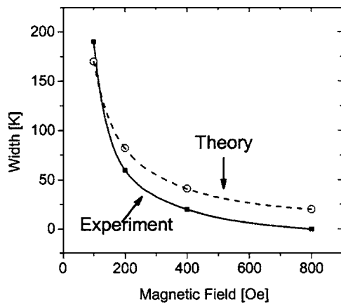
FIG. 3. Width (temperature interval between the minima) of the thermal hysteresis as a function of the external field for 2 nm \text{Co}_{0.8}\text{Gd}_{0.2} alloy. The theory for \text{Co}_{0.772}\text{Gd}_{0.228} alloy is shown by the dashed line.
