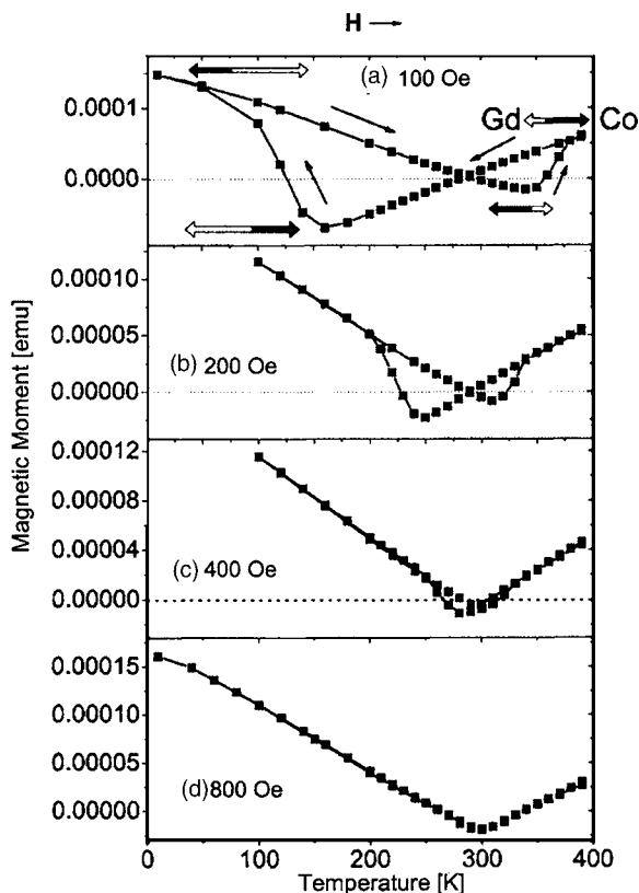
FIG. 1. Thermal hysteresis with increasing external magnetic fields for 2-nm-thick \text{Co}_{0.8}\text{Gd}_{0.2} alloy. The Co and Gd magnetization directions are shown as black and white arrows, respectively. The external magnetic field, H , points to the right as shown.
