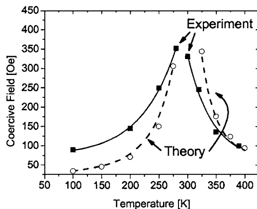
FIG. 4. Coercive field as a function of temperature for 2 nm \text{Co}_{0.8}\text{Gd}_{0.2} alloy, experiment and theory ( \text{Co}_{0.772}\text{Gd}_{0.228} ) are both shown.
