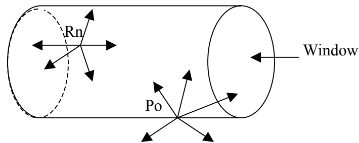
Figure (2): A typical cylindrical cell used for grab sampling. A glass window on the right is not covered with scintillation material. For simplicity, the fittings used to fill the cell are not shown. A typical radon-222 atom is shown within the air inside the cell. The arrows represent possible paths for the alpha particle released by the radon. A typical polonium-218 or polonium-214 atom is shown plated out on the bottom right of the interior of the cell. Theoretical paths for its alpha are also shown with arrows. Of course, alpha particles can not penetrate the walls of the cell and such paths would be counted as hits, or flashes.
