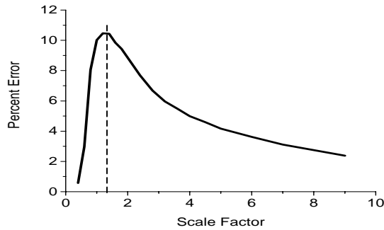
Figure (3): Percent error versus scale factor the Rocky Mountain cell geometry. The scale factor gives the increase or decrease in both the height and diameter from the original cell geometry.
