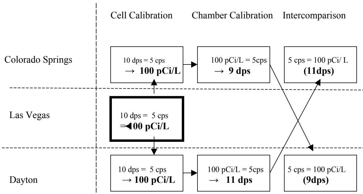
Figure (1): A block diagram showing calibration of cells stage (left), subsequent calibration of chambers from the cells (middle) and, lastly, intercomparison of radon in the chamber using cells filled at each site.
